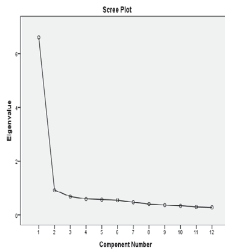
Figure 1. Scree Plot
