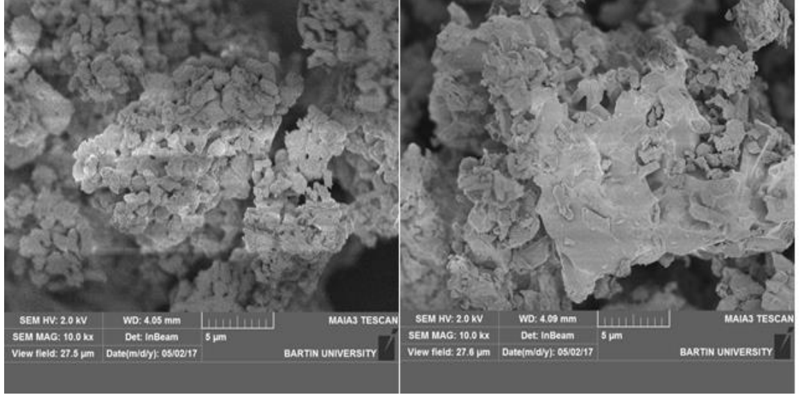
Saf Mg_2B_2O_5
