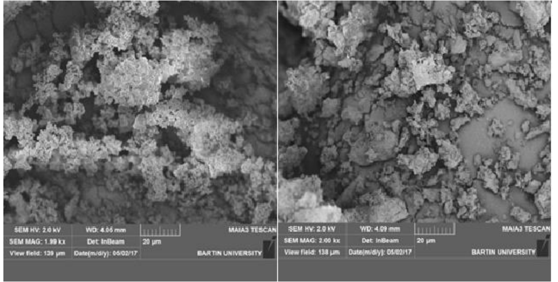
Saf Mg_2B_2O_5
